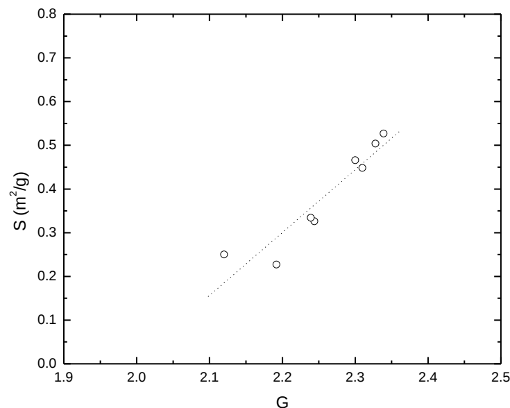
Fig. 4: The relationship between specific gravity and specific surface area of fly ashes
