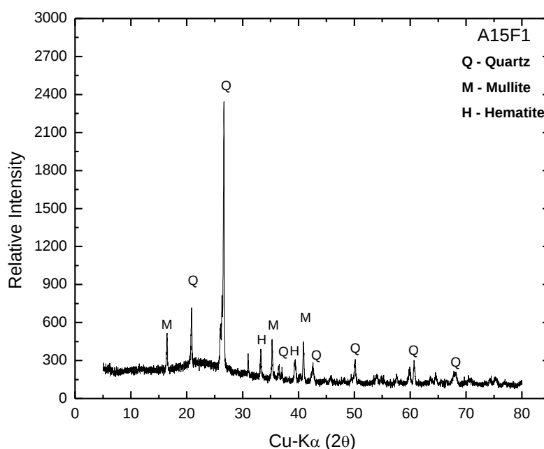
Fig. 6: A typical X-ray diffractogram of a fly ash sample
