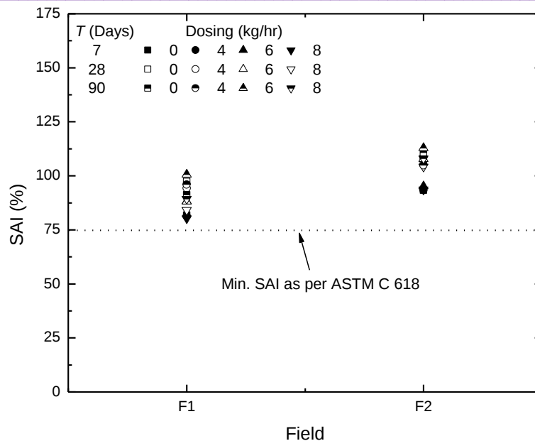
Fig. 3: Strength activity index of fly ash samples
