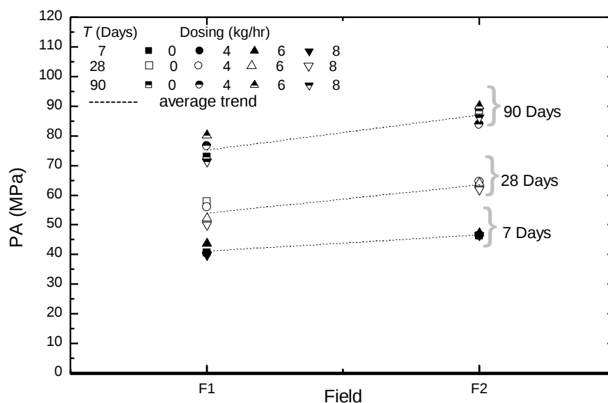
Fig. 2: Pozzolanic activity of fly ash samples
