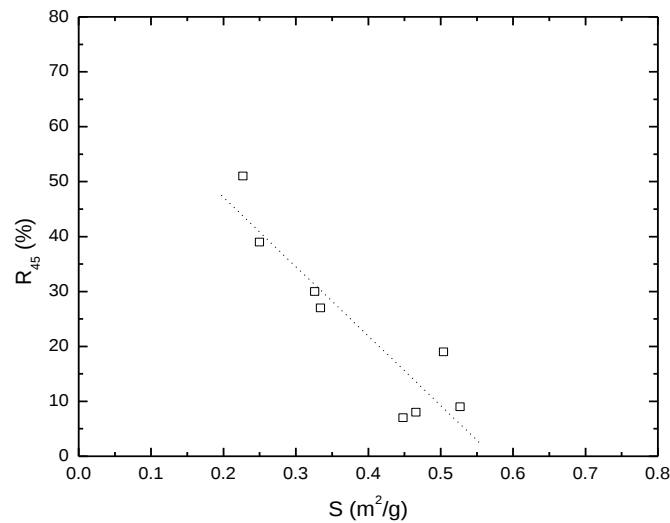
Fig. 5: The relationship between specific surface area and R_{45} of fly ashes
