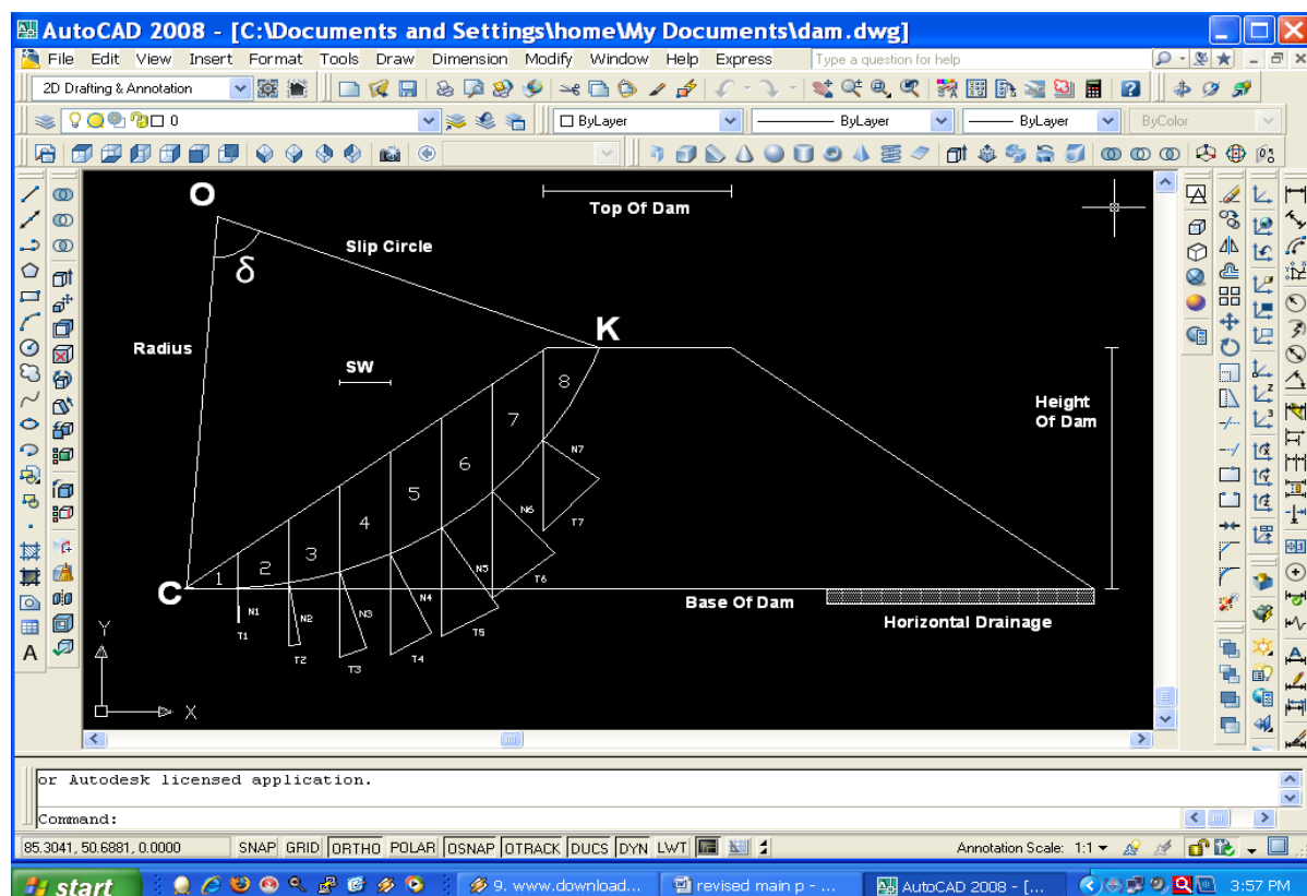
Fig. 2.1 Swedish Slip Circle Method.
