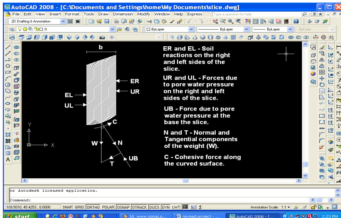
Fig. 2.2 Different Forces Acting on the Slice.
