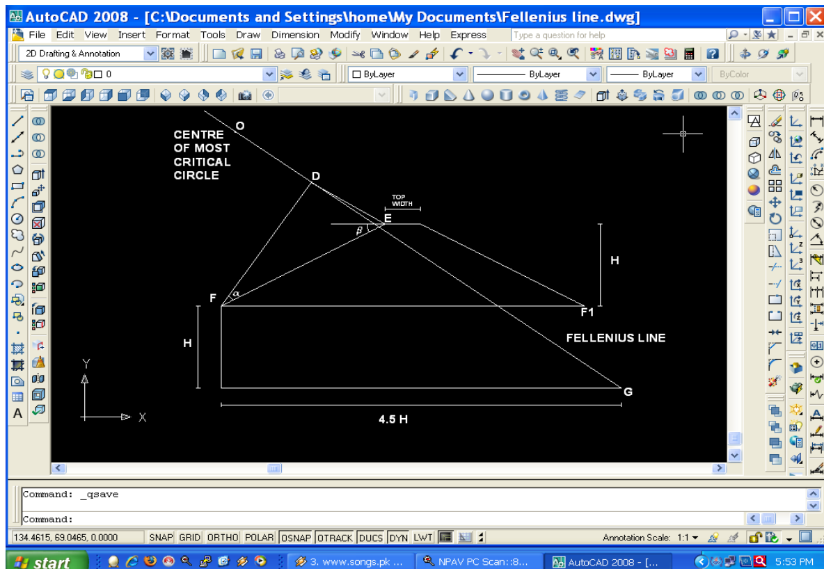
Fig. 2.4 Location of the Most Critical Circle.
