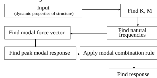
Fig. 3 Flow Chart for RSA.
