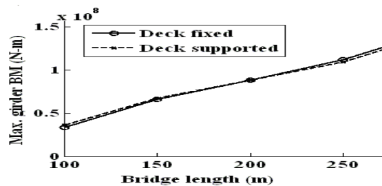
Fig. 12 Effect on Deck BM.
