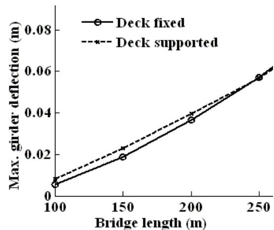
Fig. 5 Effect on Deck Deflection.
