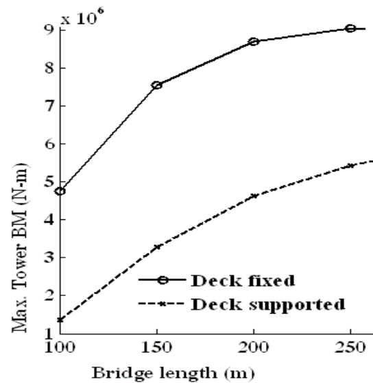
Fig. 13 Effect on Tower BM.
