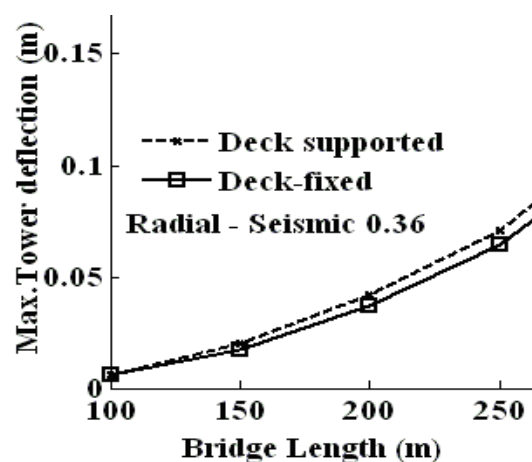
Fig. 11 Effect on Tower Deflection for z = 0.36 .
