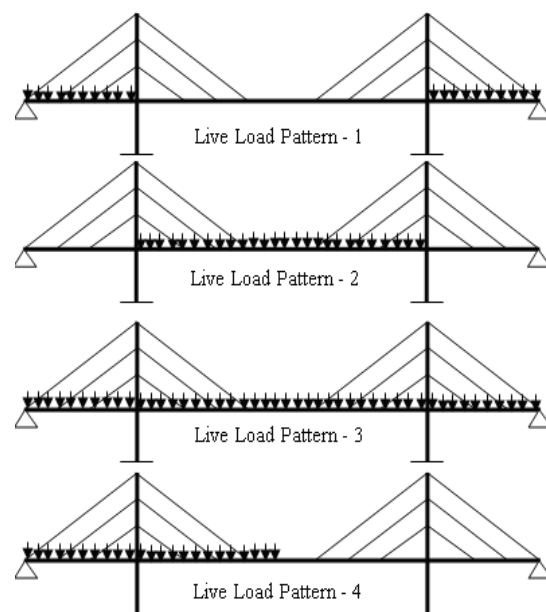
Fig. 2 Live Load Patterns on Bridge.
