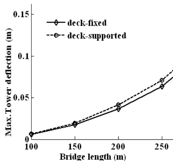
Fig. 6 Effect on Tower Deflection.
