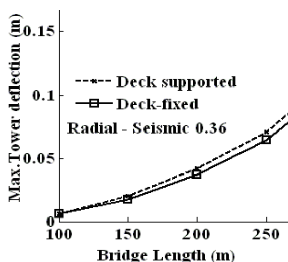
Fig. 8 Effect on Tower Deflection for z = 0.36 .
