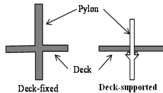
Fig. 1 Deck-Pylon Connection Details.
